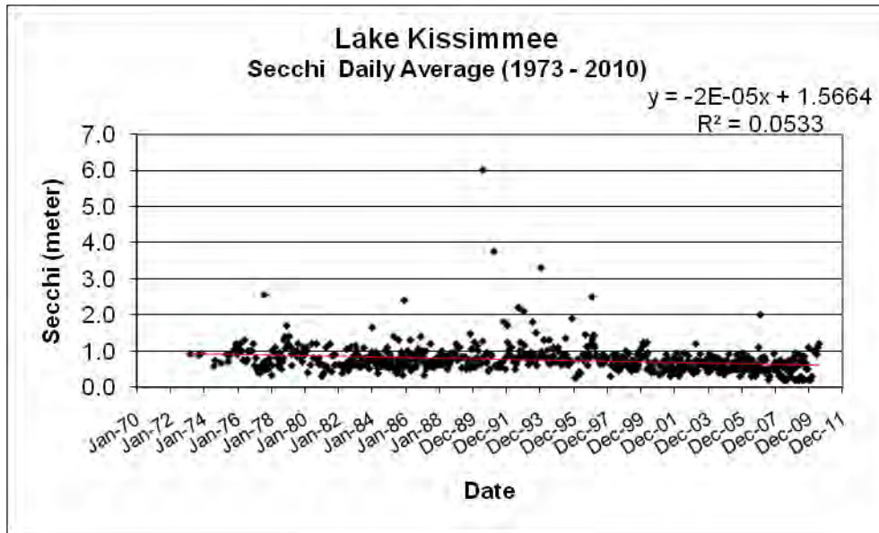
Figure 2.5 Daily Average Secchi (meters)
