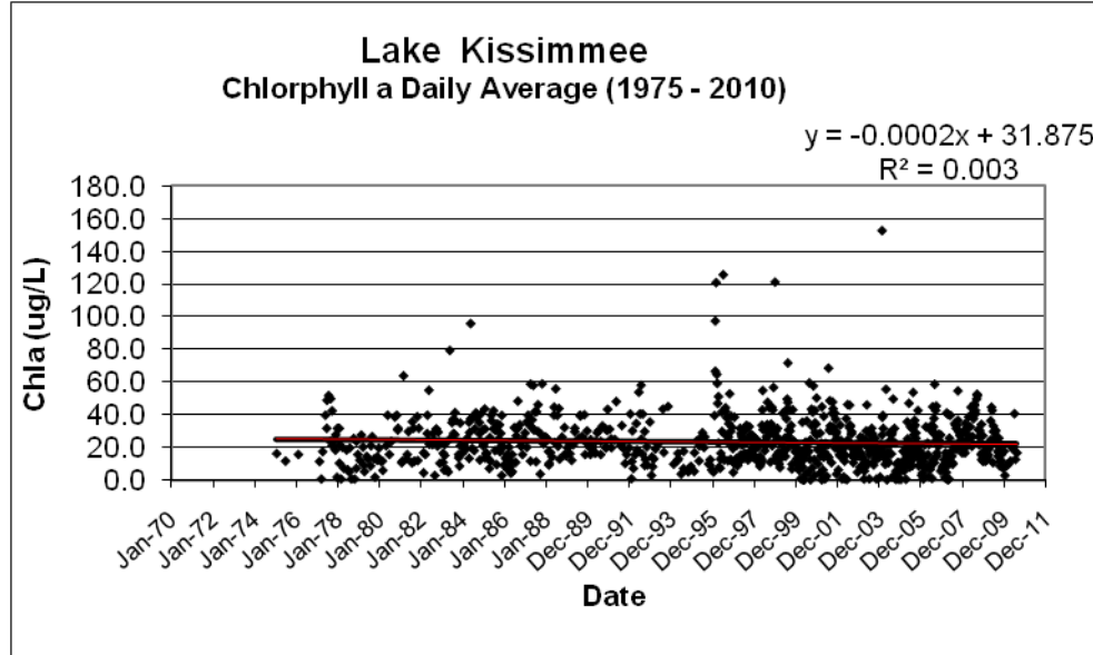
Figure 2.15 Corrected Chlorophyll a Daily Average Results
