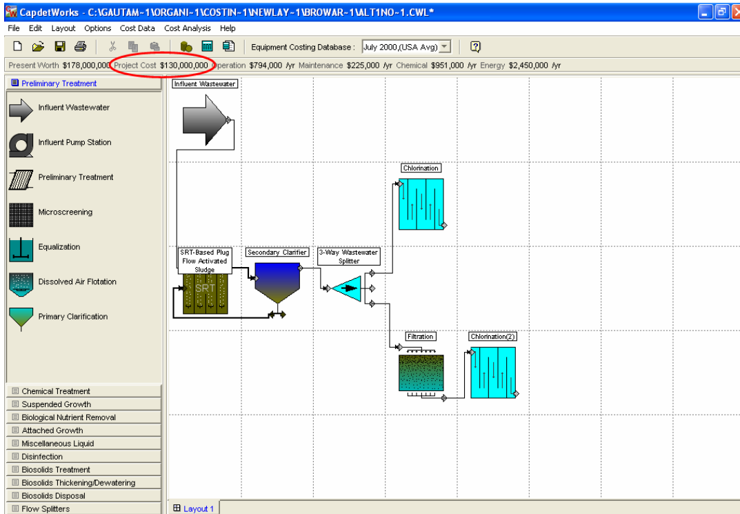
Appendix Figure 1-9. Project Cost of treatment process for Broward/North WWTP 2005 Flow with Alternative 1, scenario A, as evaluated by CapdetWorks
