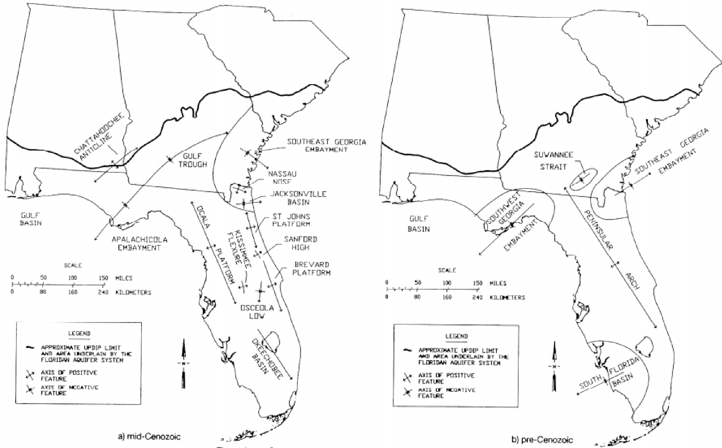
Figure 4. Structural features of Florida: a) mid-Cenozoic b) pre-Cenozoic
