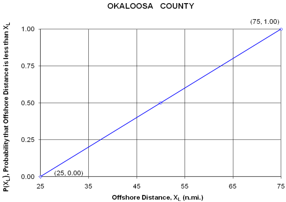
Figure 7 Cumulative Probability Distribution of Offshore Distance, X_L , for Alongshore Storms
