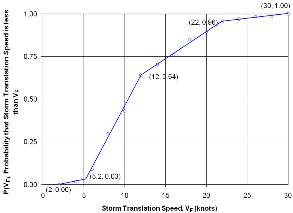
Figure 5 Cumulative Probability Distribution of Translation Speed, V_F
