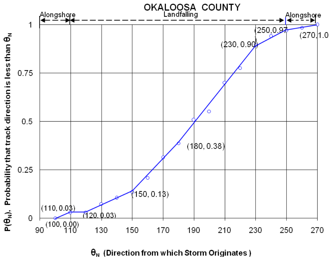
Figure 1 Cumulative Probability Distribution of Storm Track Direction, \theta_N
