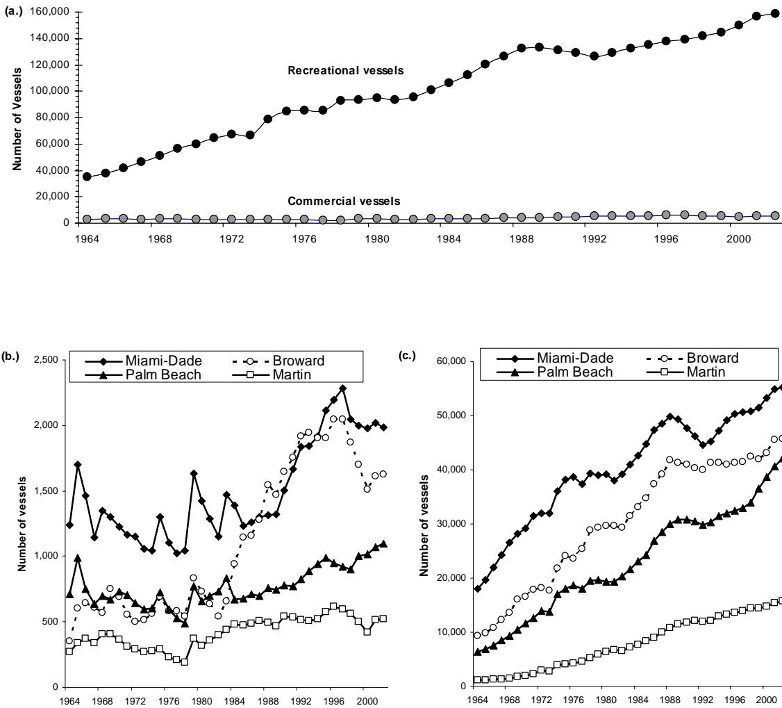
Figure 4. Trends in total registered vessels in the SEFCRI region, 1964-2001. (a.) Total number of registered recreational and commercial vessels. (b.) Number of registered commercial vessels by county. (c.) Number of registered recreational vessels by county.
