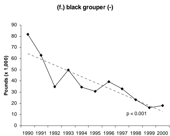
Figure 18. Commercial landings of major reef fishes in SEFCRI region 1990-2000 (a.) greater amberjack, (b.) yellowtail snapper, (c.) mutton snapper, (d.) gag grouper, (e.) blue runner, (f.) black grouper. Dotted lines show significant ( p < 0.05 ) linear trends.
